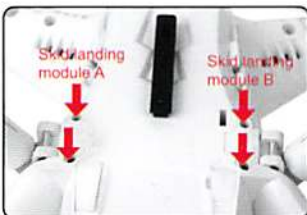
2.2.3 Install the skid landing module, and screw down the M2.5X20 screw to fix skid landing.
