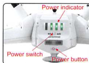
2.1.4 Turn the power switch to "ON" position, and press on the power button about 3-5 second till the red LED light solid. The undercarriage(skid landing) will unfold automatically.
