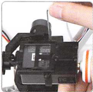
3.4 Install the camera to the Gimbal, fix it with the camera fixing frame (make sure the gap close to the lens), then use 2 M2X4 screws to tighten the camera fixing frame.
