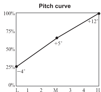
Autorotation landing
